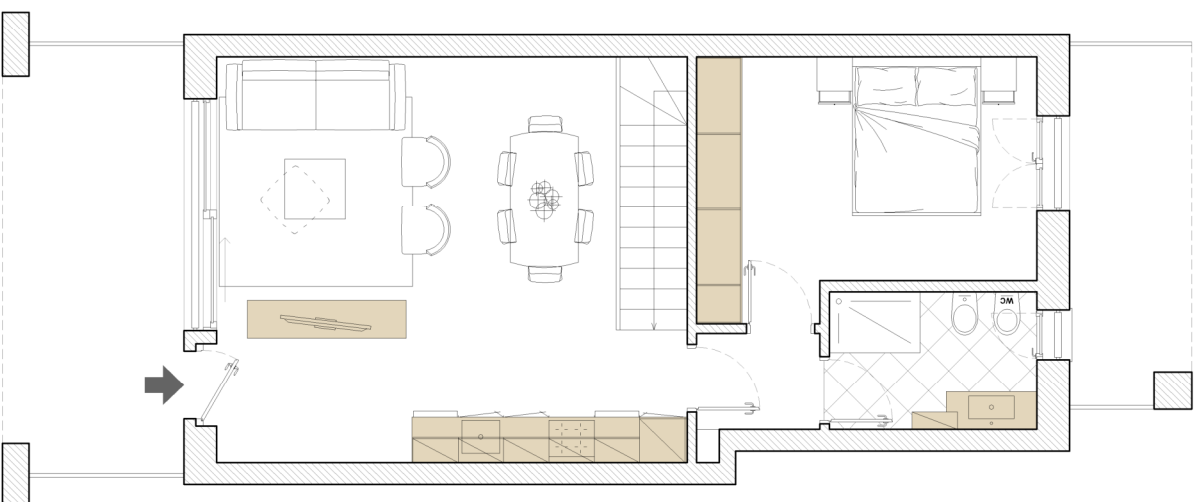
PIANO TERRA
